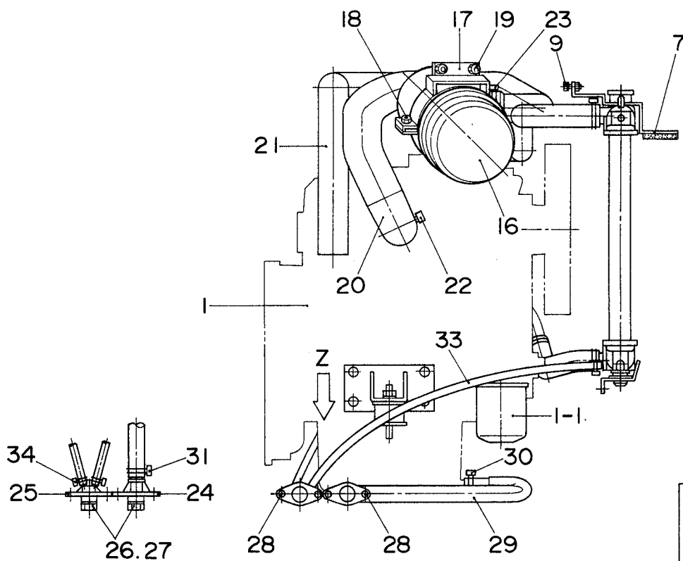
VIEW - Z
